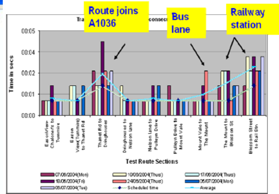
Figure 5b. Typical calibration outputs
