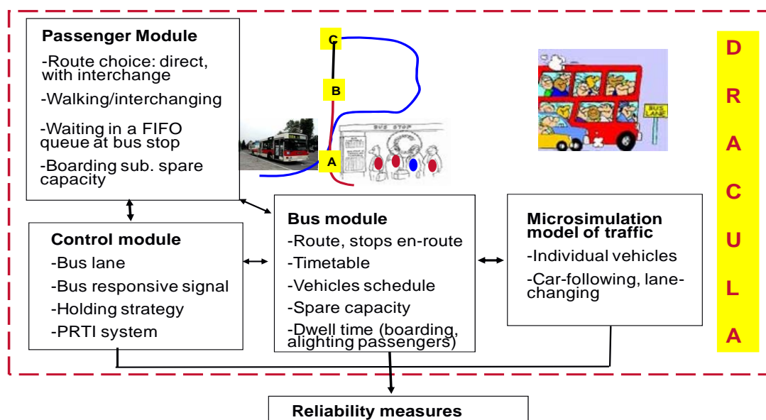
Figure 4. A modelling framework to represent public transport operations
